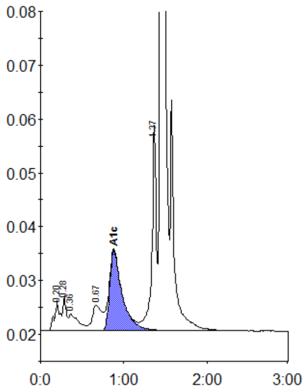
Peak table - ID: 10411313
